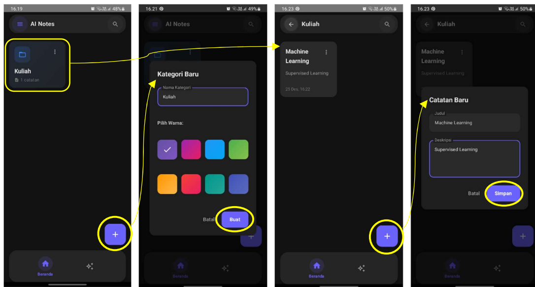
Gambar 7 Main Screen
