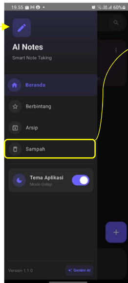
Gambar 19 Drawer Menu
