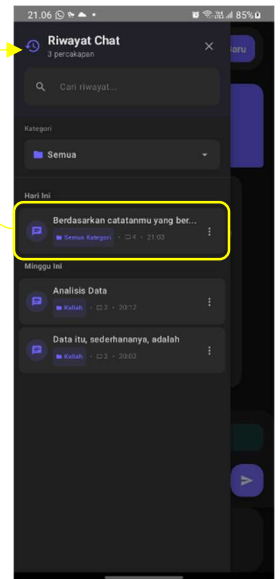
Gambar 30 History Chat
