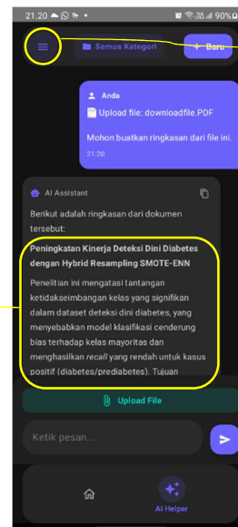
Gambar 34 Hasil Summary
