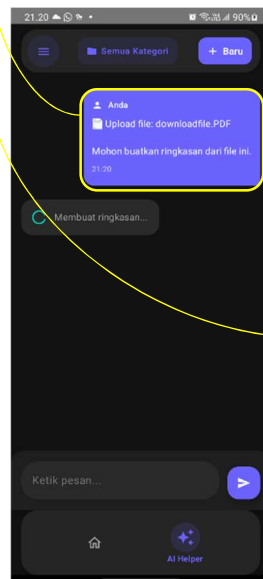
Gambar 33 Proses Summary
